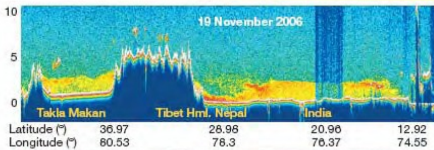
CALIPSO data for BC surrounding Himalayas
